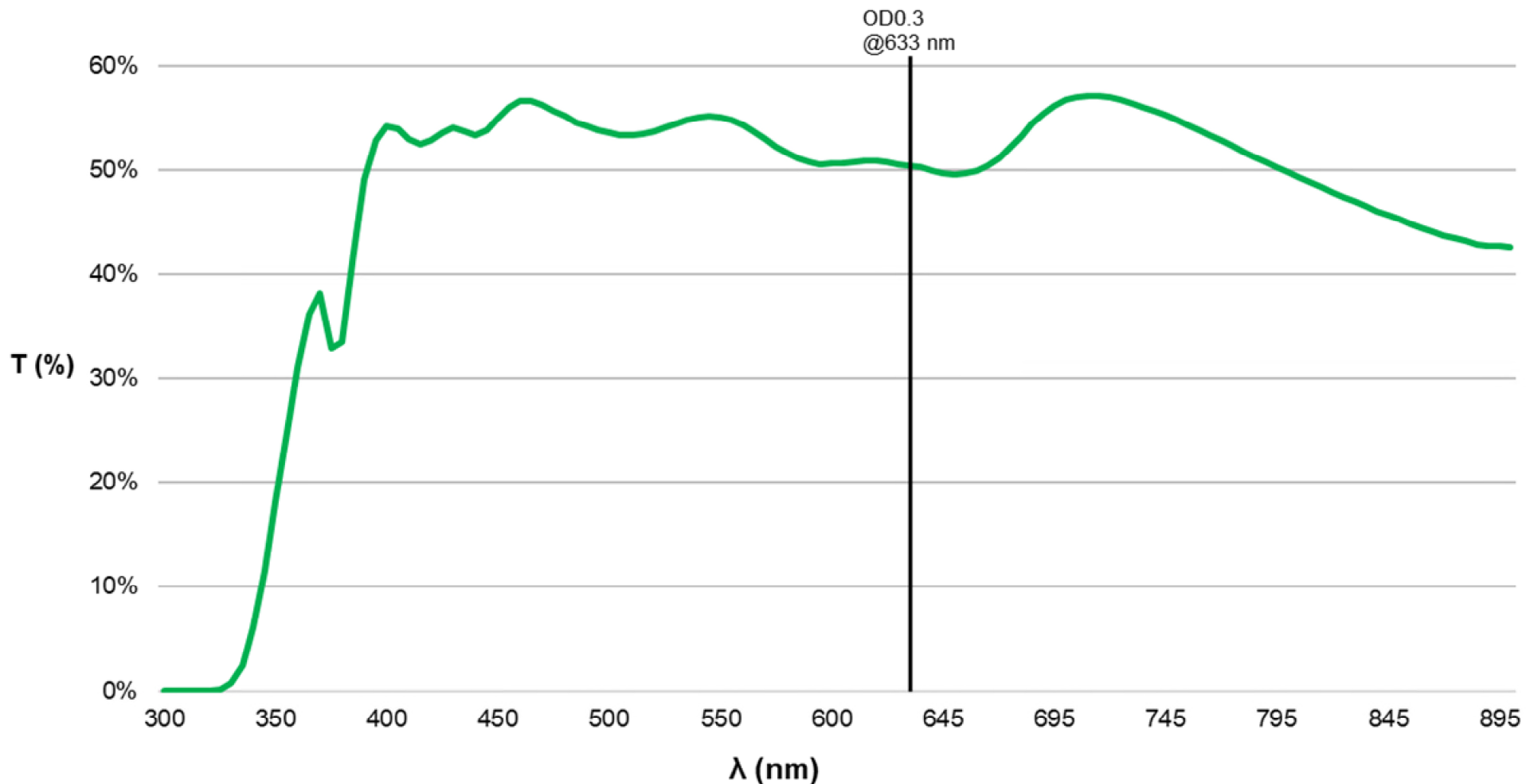
SCHOTT NG11 633 nm 50 Sq., 0.3 OD ND Filter REFERENCE Only
