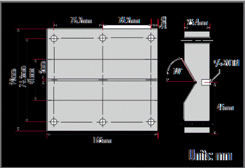
V-Block Base
