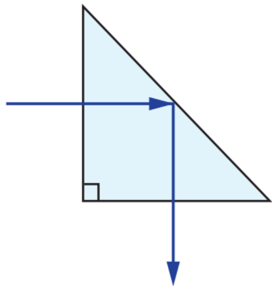
Right Angle Prism Ray Path
