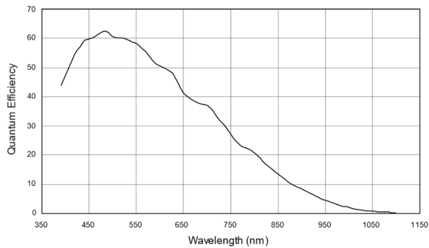
MT9P031 Sensor QE Curve
