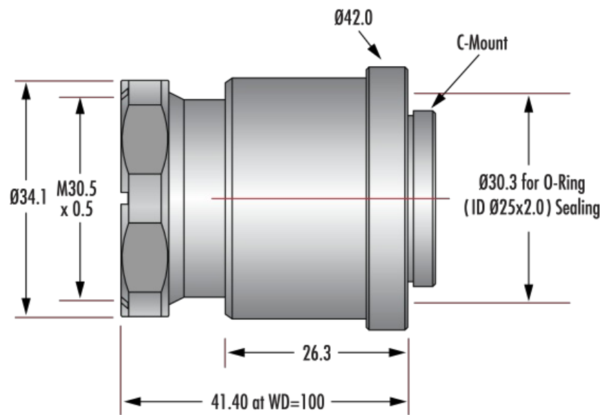
25mm Cw Series Fixed Focal Length Lens
