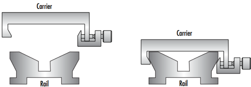
Side Profile of Rail System
